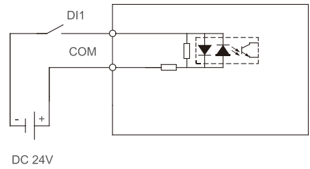
NPN signal input wiring when using external DC24V power supply
