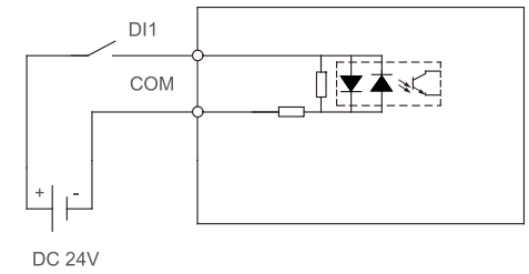
PNP signal input wiring when using external DC24V power supply
