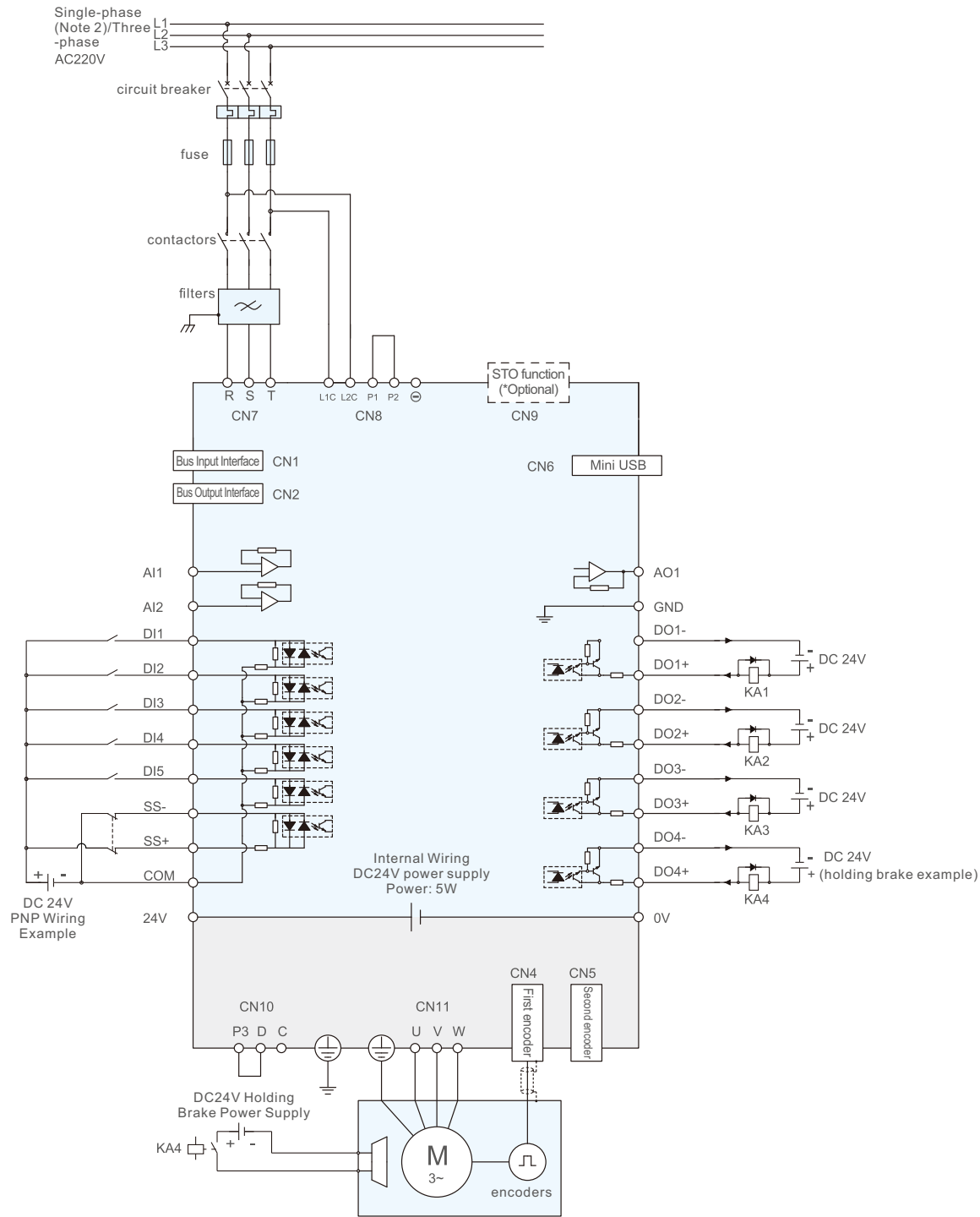
AC220V class A3 specification standard type AD2 Drive Wiring Diagram
